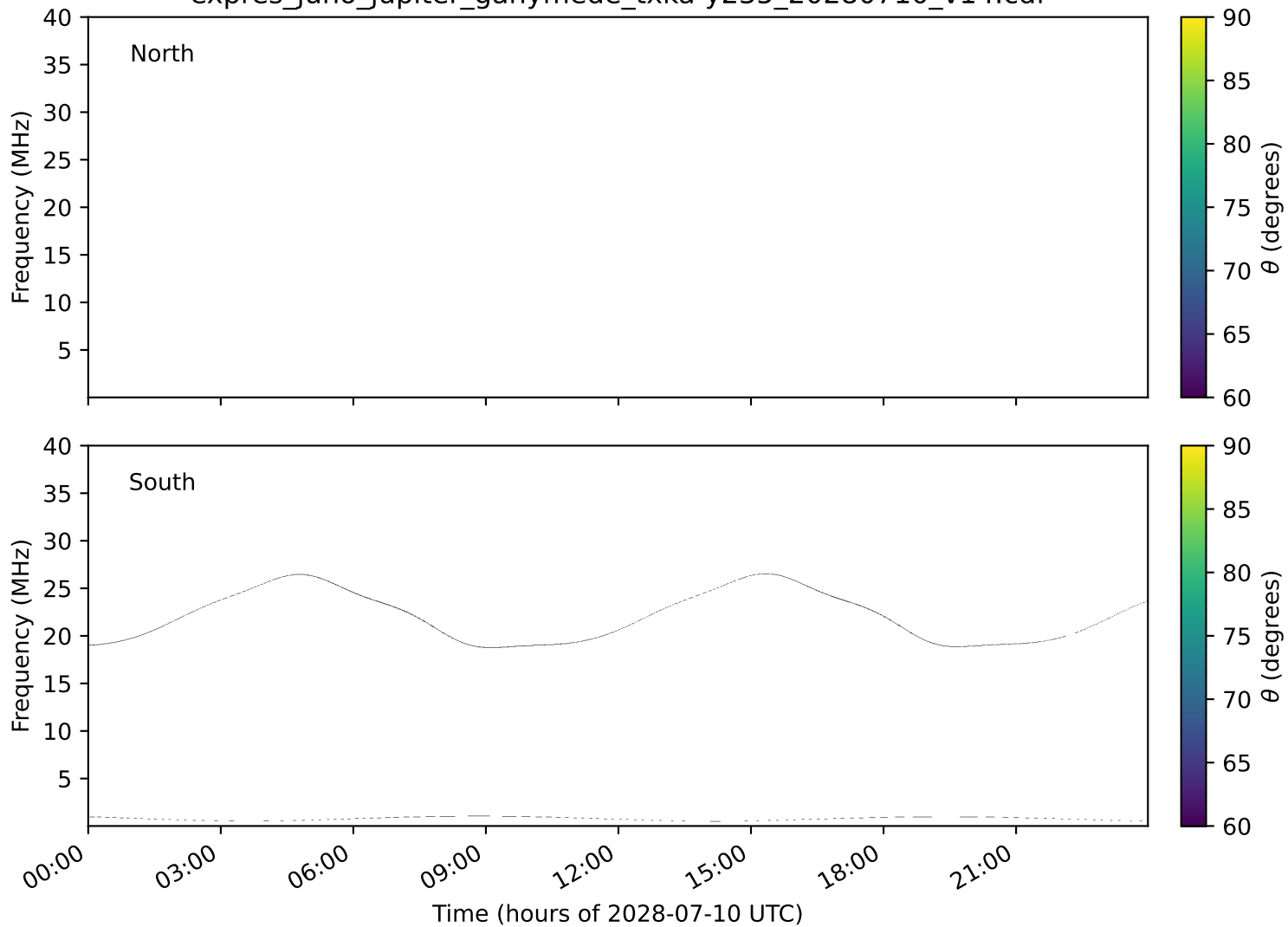
expres_juno_jupiter_ganymede_txka-y235_20280710_v14.cdf
