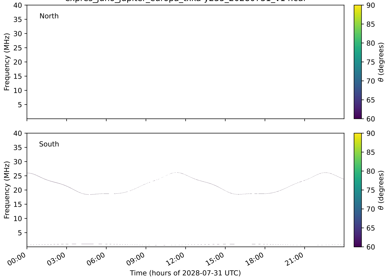
expres_juno_jupiter_europa_txka-y235_20280731_v14.cdf
