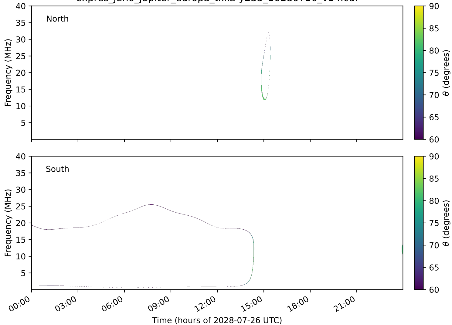
expres_juno_jupiter_europa_txka-y235_20280726_v14.cdf
