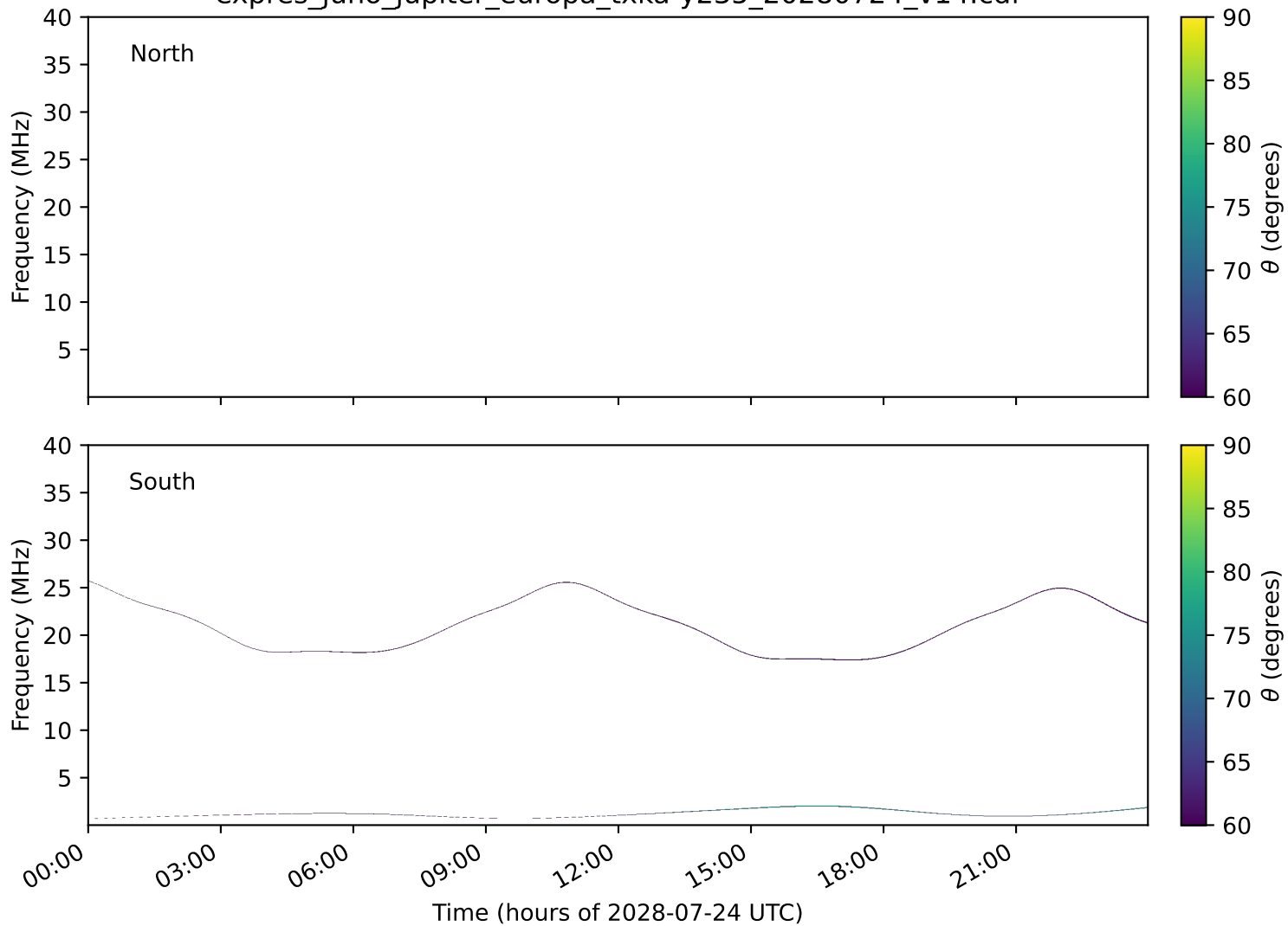
expres_juno_jupiter_europa_txka-y235_20280724_v14.cdf
