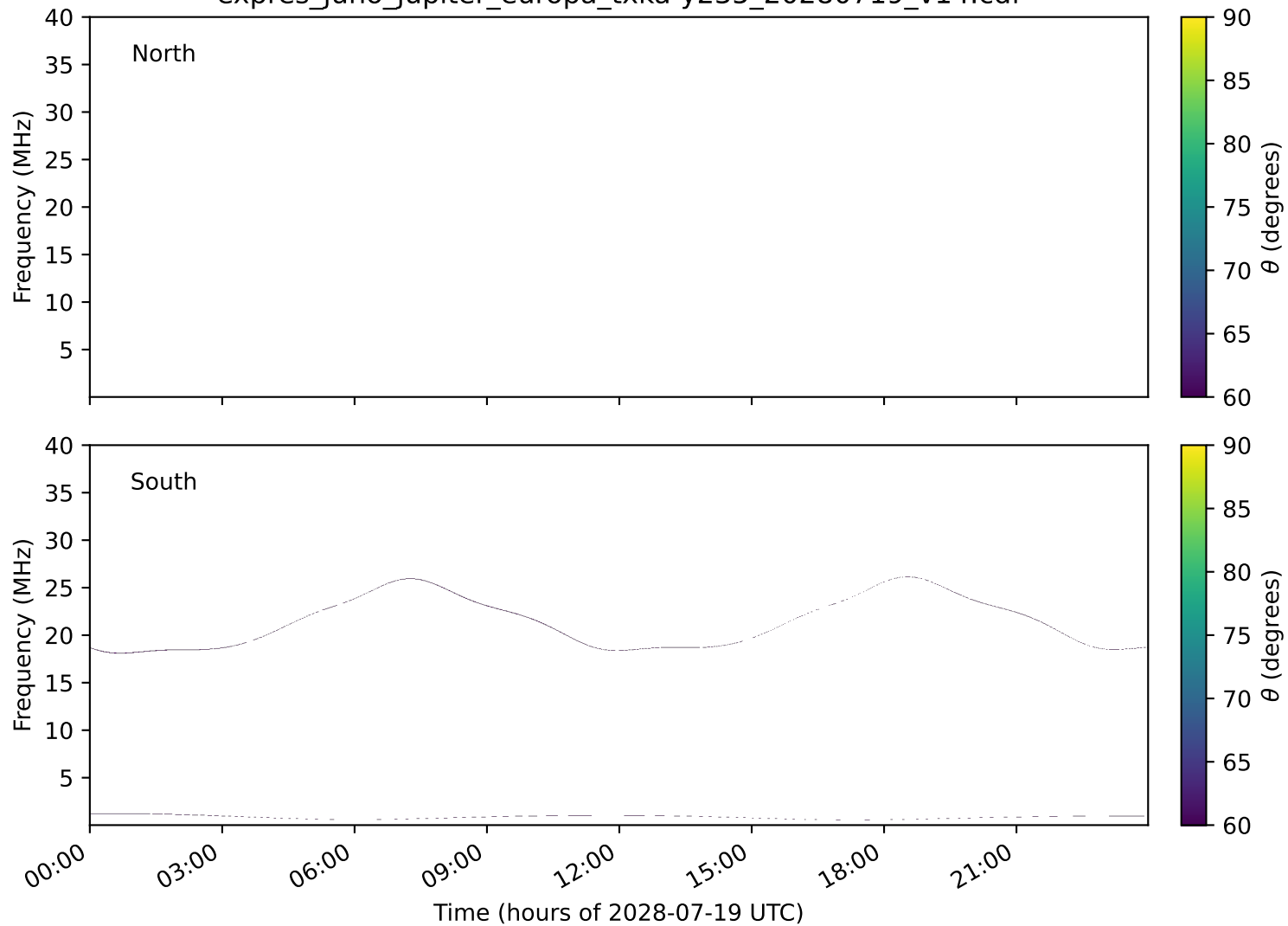
expres_juno_jupiter_europa_txka-y235_20280719_v14.cdf
