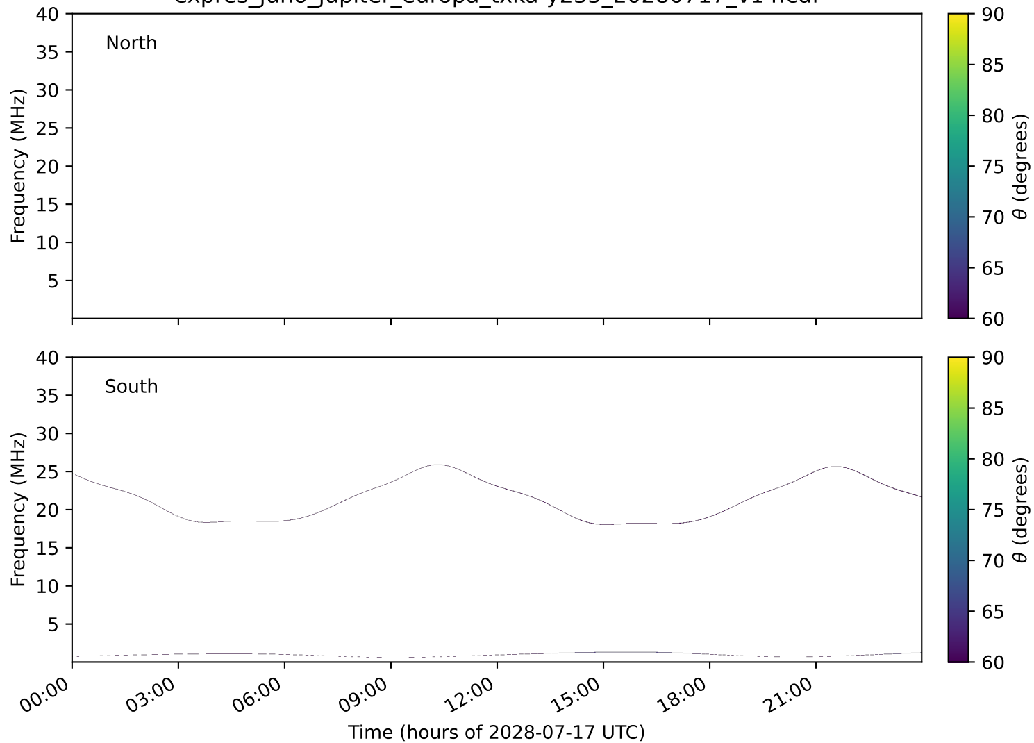
expres_juno_jupiter_europa_txka-y235_20280717_v14.cdf
