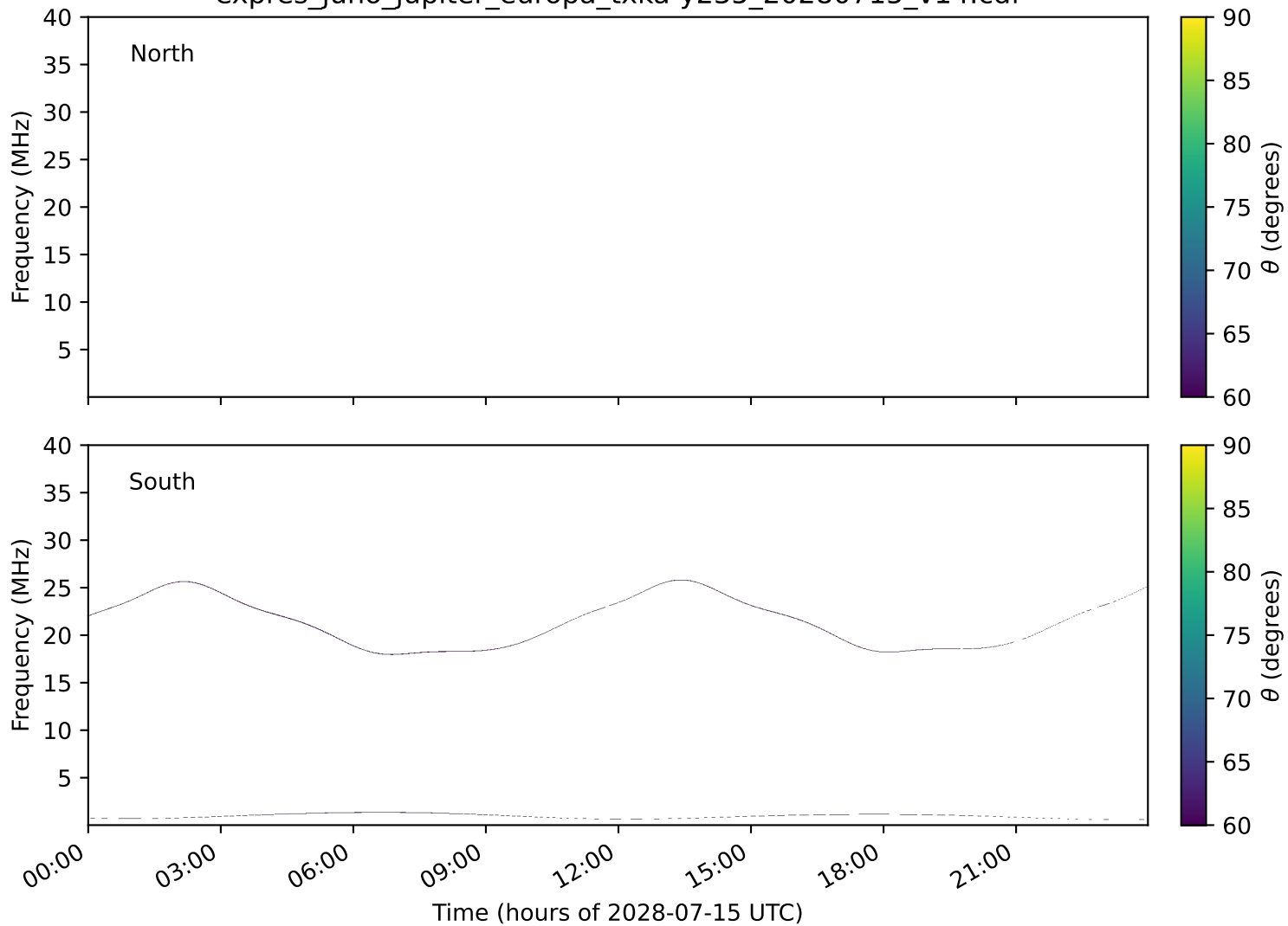
expres_juno_jupiter_europa_txka-y235_20280715_v14.cdf
