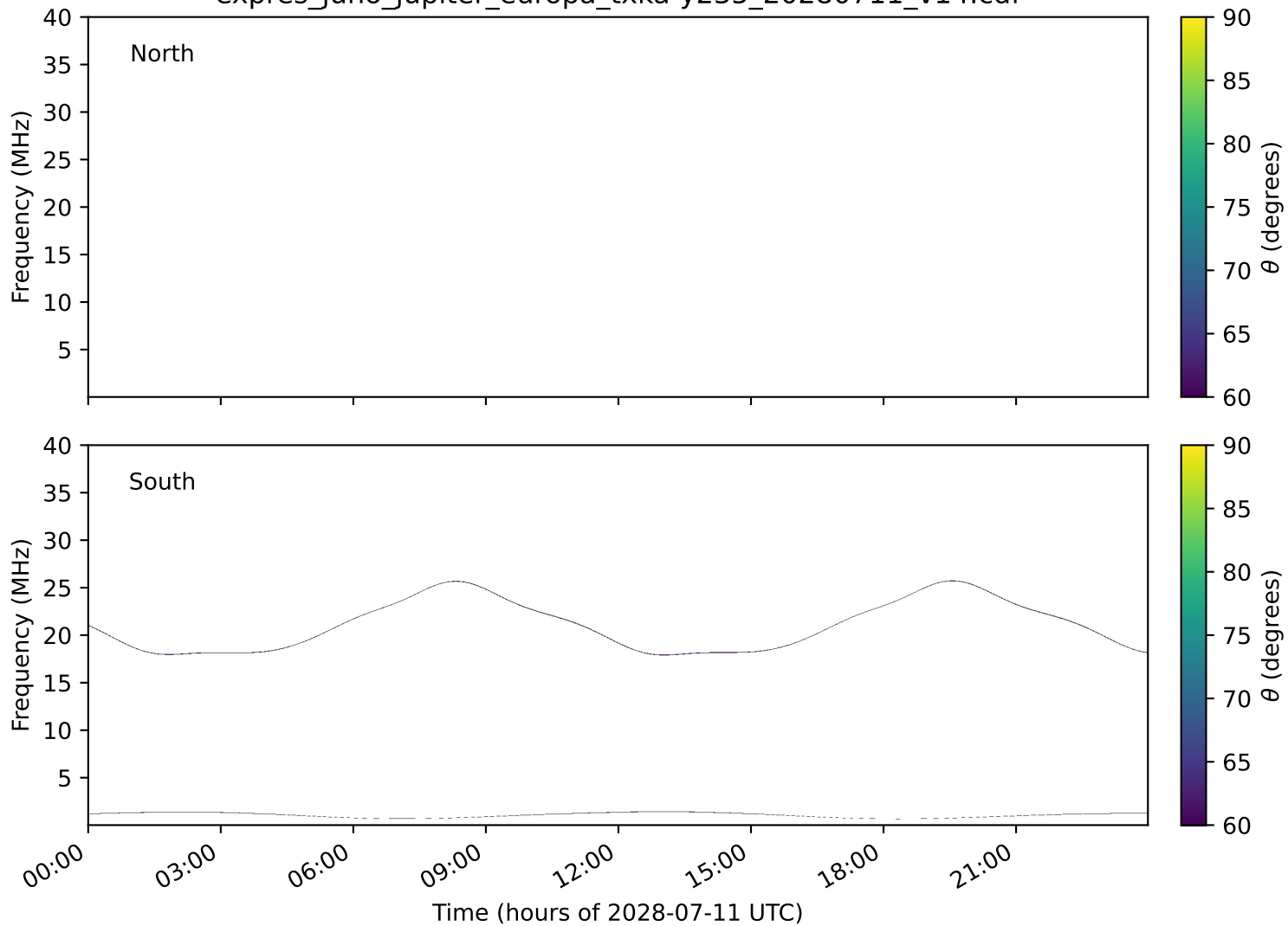
expres_juno_jupiter_europa_txka-y235_20280711_v14.cdf
