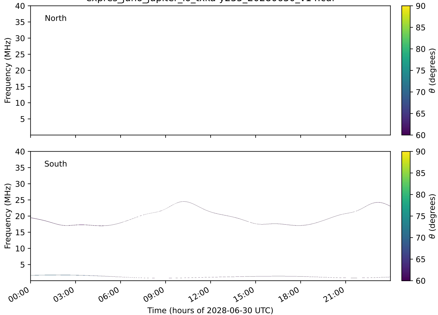
expres_juno_jupiter_io_txka-y235_20280630_v14.cdf
