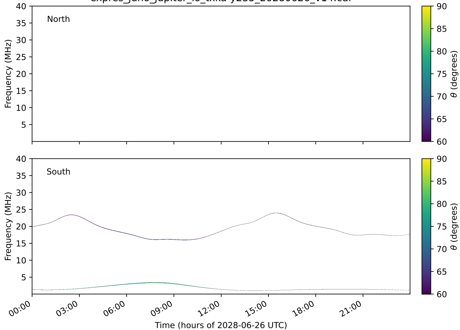
expres_juno_jupiter_io_txka-y235_20280626_v14.cdf
