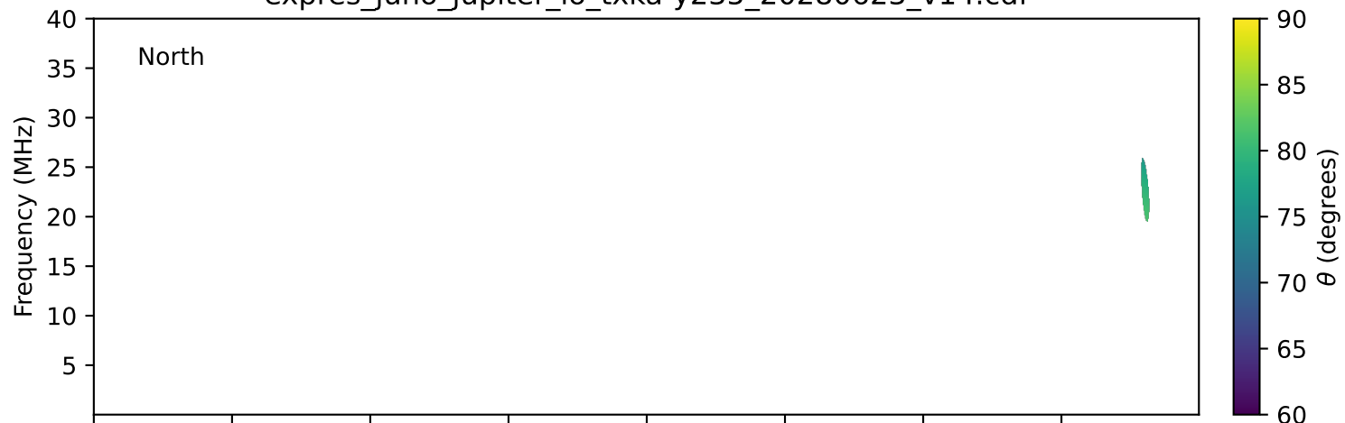
expres_juno_jupiter_io_txka-y235_20280623_v14.cdf
