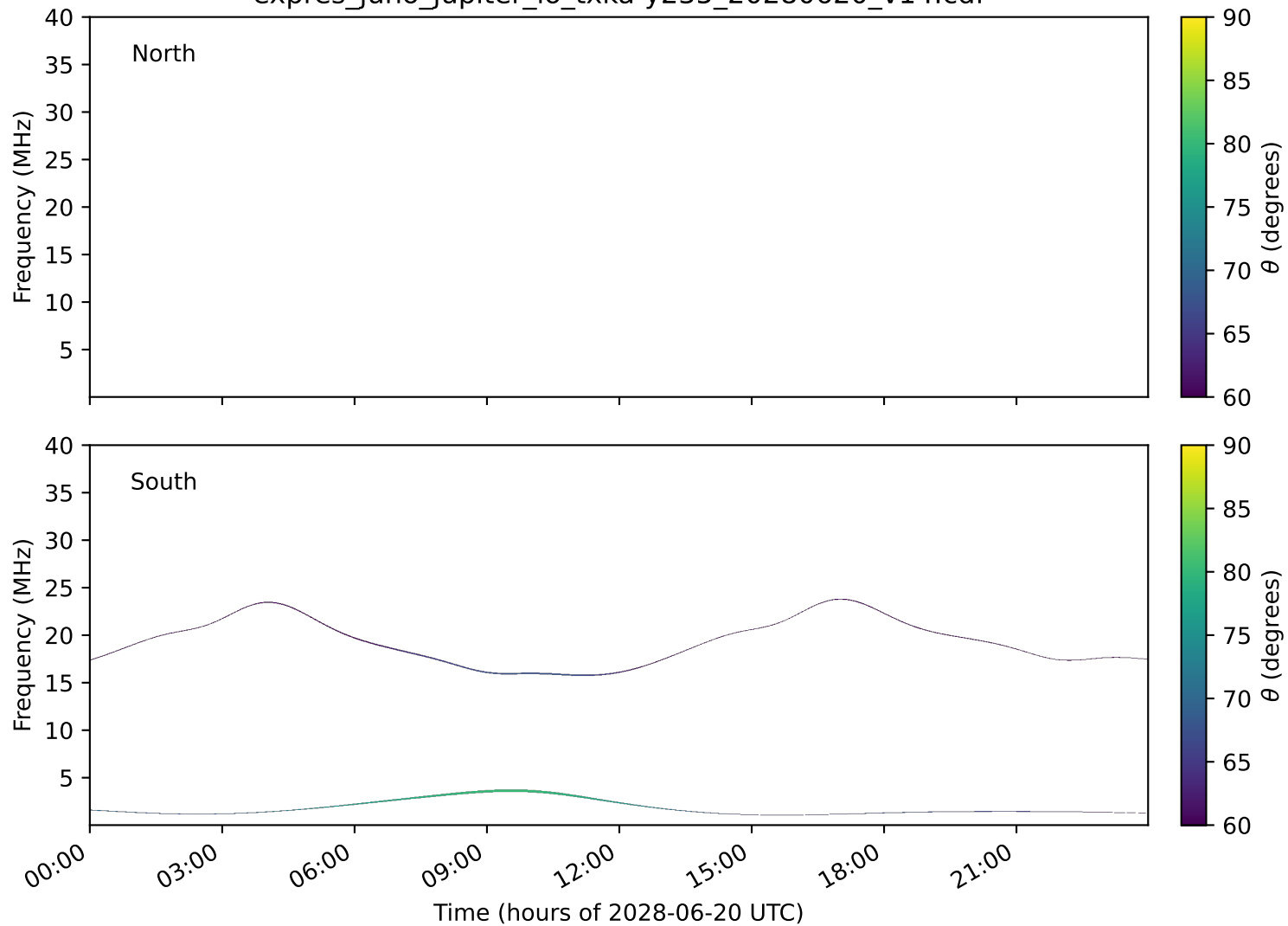
expres_juno_jupiter_io_txka-y235_20280620_v14.cdf
