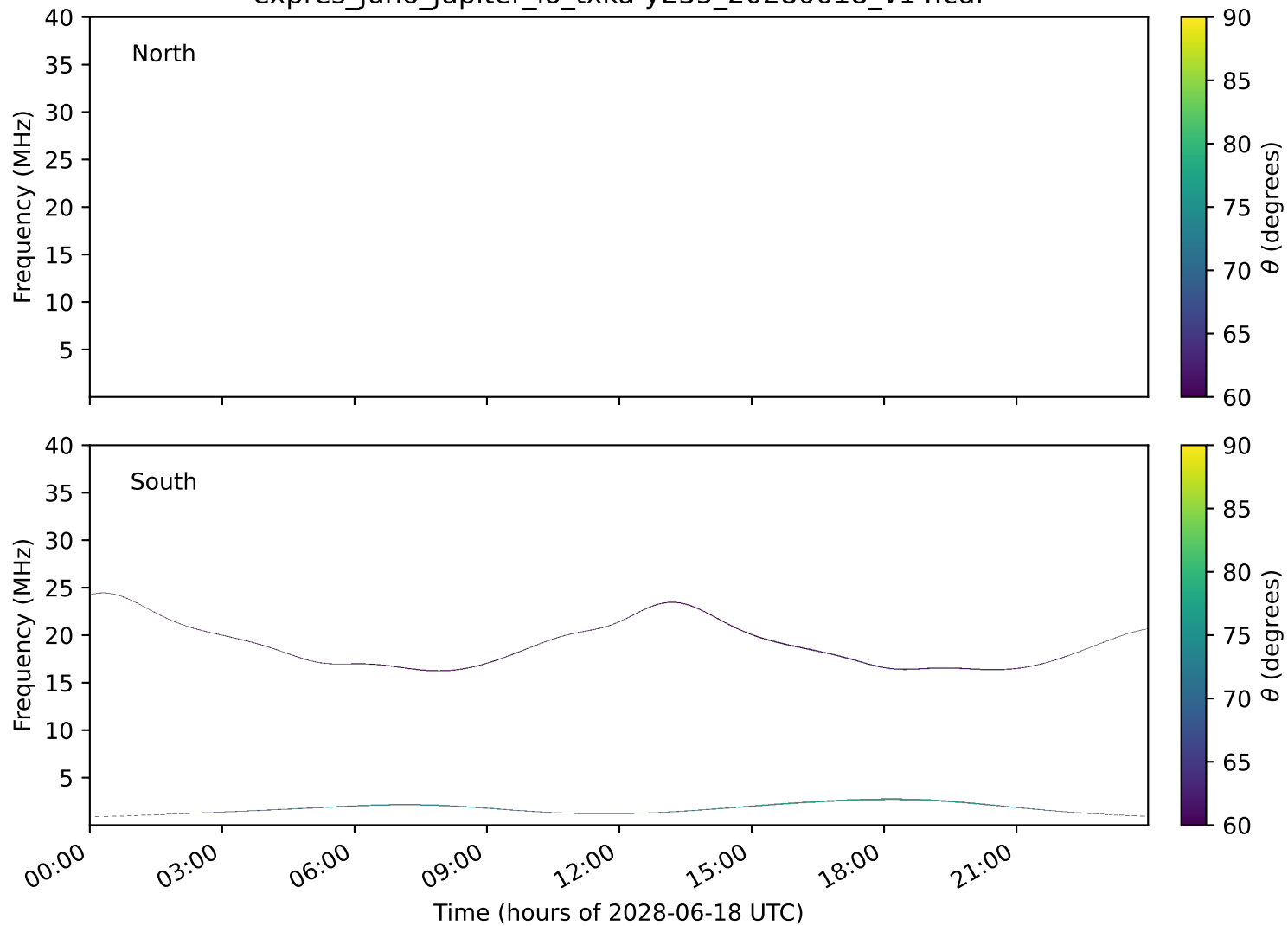
expres_juno_jupiter_io_txka-y235_20280618_v14.cdf
