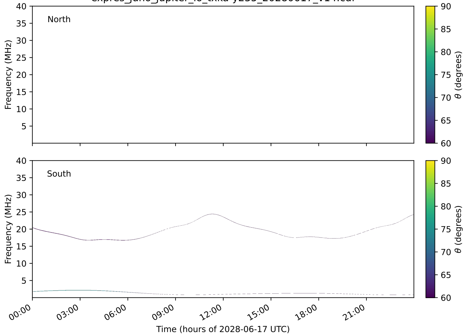
expres_juno_jupiter_io_txka-y235_20280617_v14.cdf
