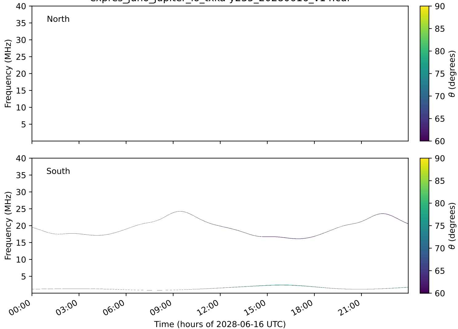
expres_juno_jupiter_io_txka-y235_20280616_v14.cdf
