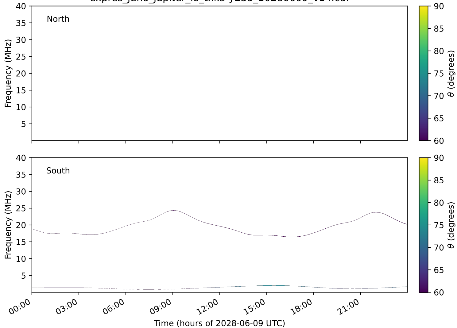
expres_juno_jupiter_io_txka-y235_20280609_v14.cdf
