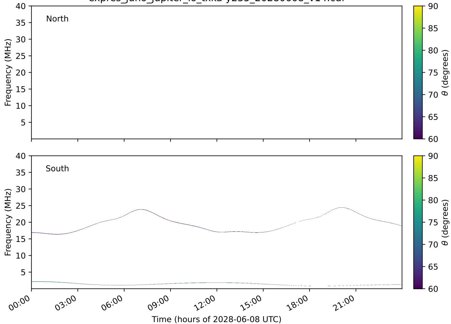
expres_juno_jupiter_io_txka-y235_20280608_v14.cdf
