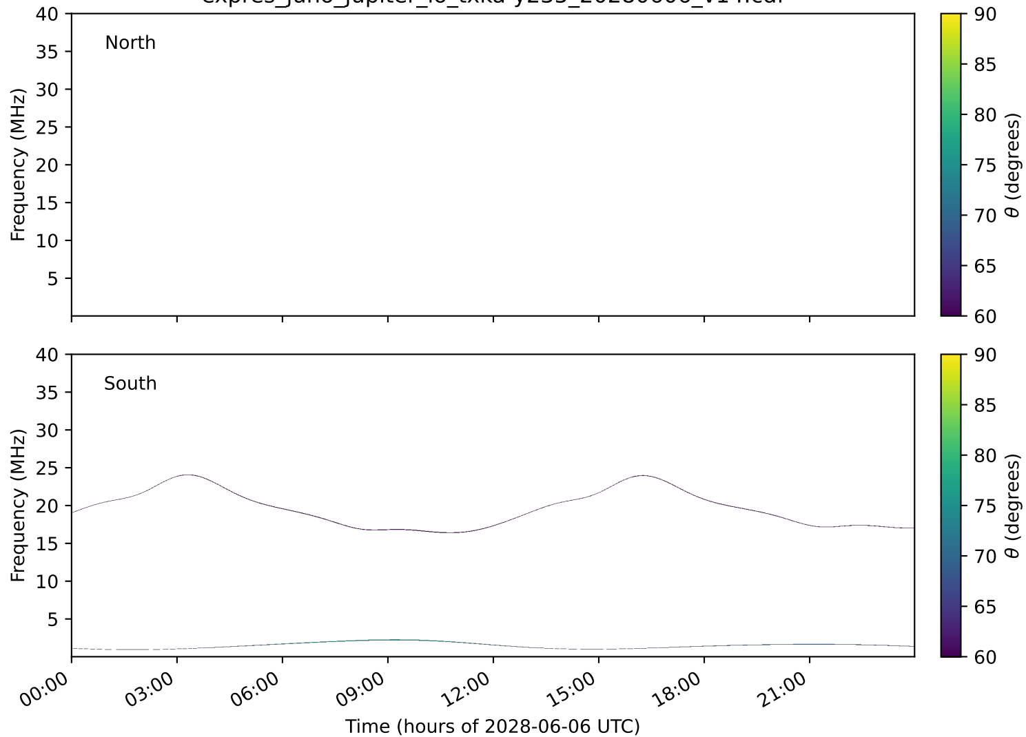
expres_juno_jupiter_io_txka-y235_20280606_v14.cdf
