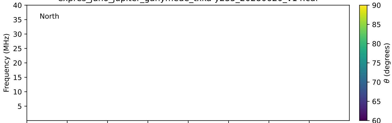
expres_juno_jupiter_ganymede_txka-y235_20280620_v14.cdf
