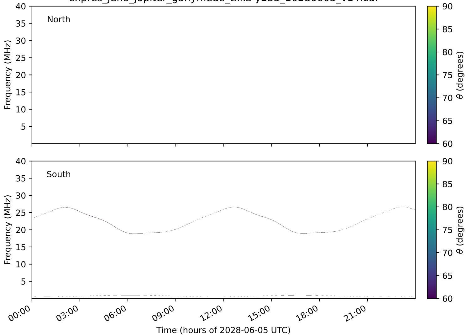
expres_juno_jupiter_ganymede_txka-y235_20280605_v14.cdf
