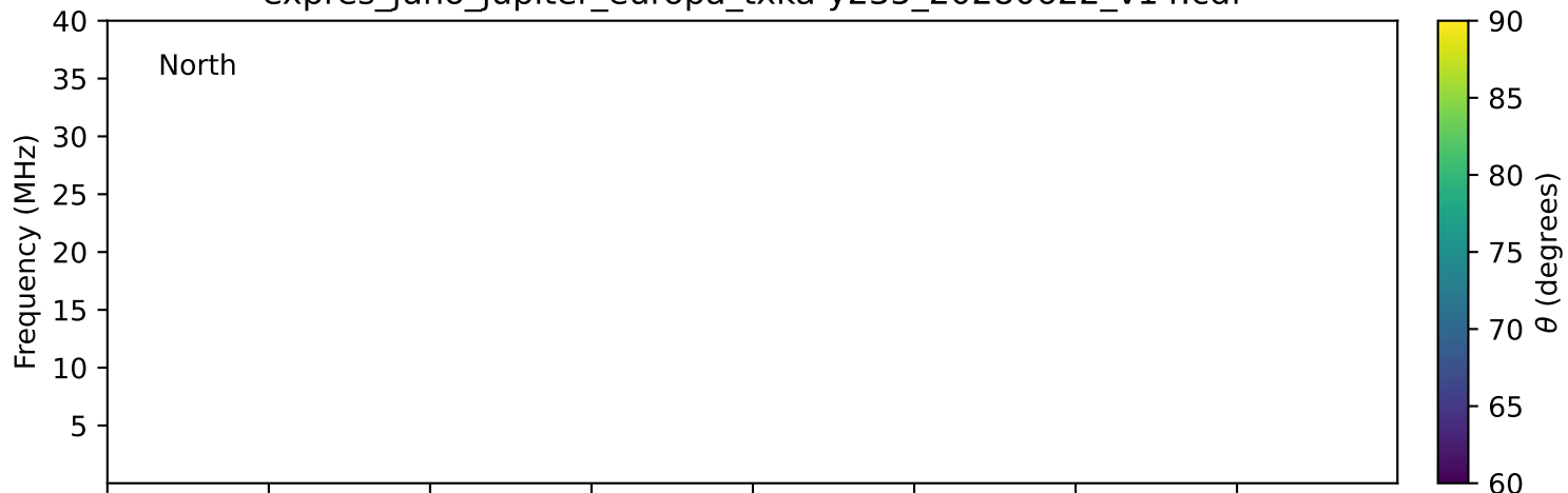
expres_juno_jupiter_europa_txka-y235_20280622_v14.cdf
