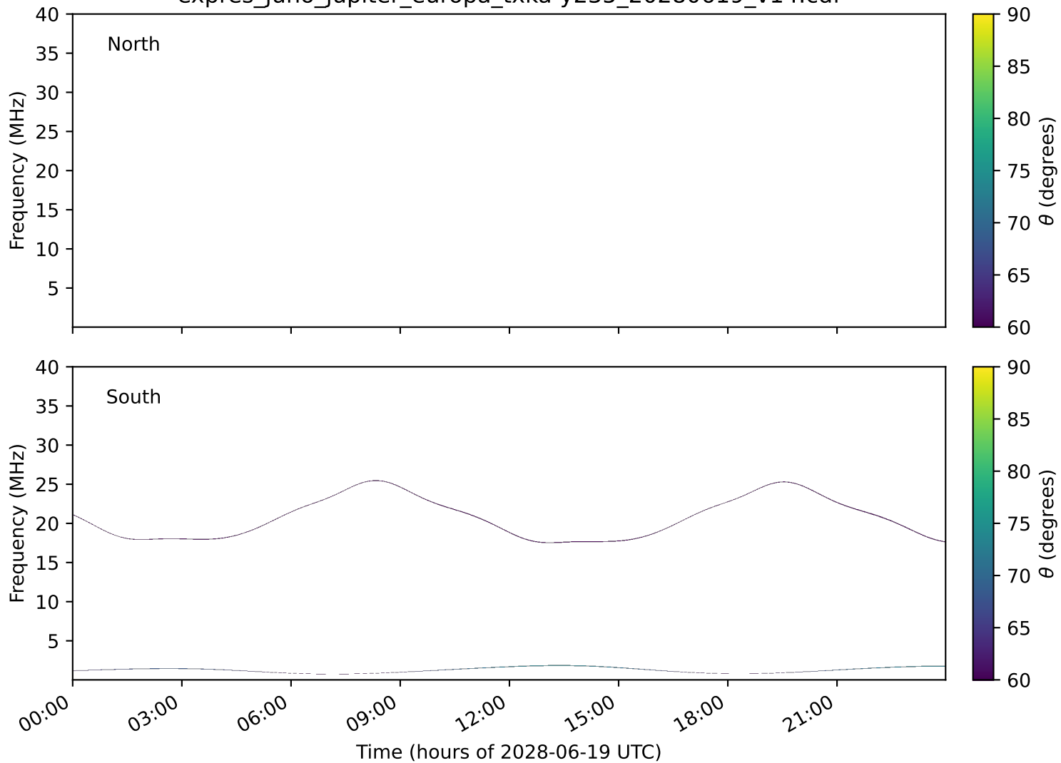
expres_juno_jupiter_europa_txka-y235_20280619_v14.cdf
