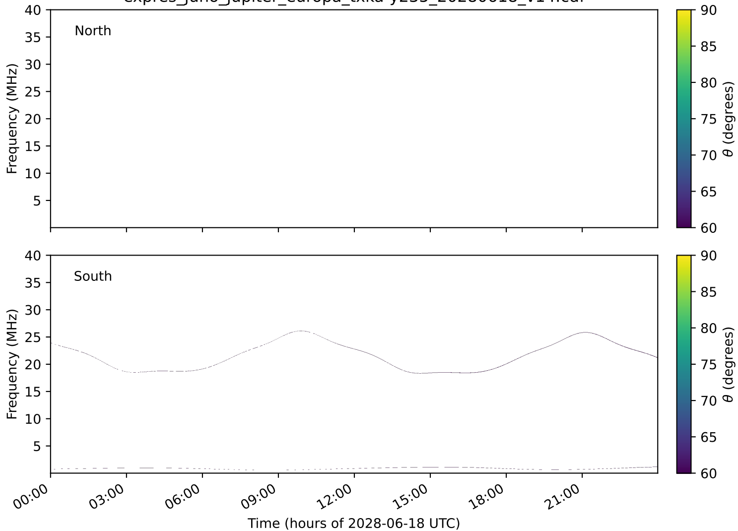
expres_juno_jupiter_europa_txka-y235_20280618_v14.cdf
