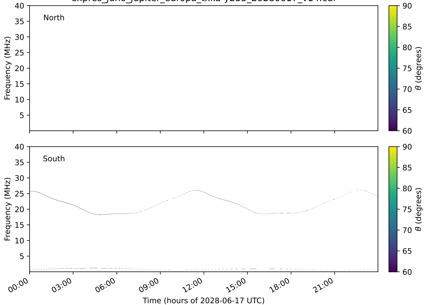
expres_juno_jupiter_europa_txka-y235_20280617_v14.cdf
