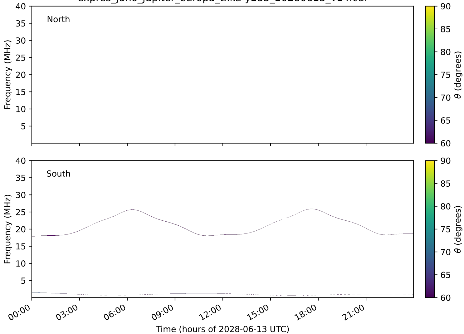
expres_juno_jupiter_europa_txka-y235_20280613_v14.cdf
