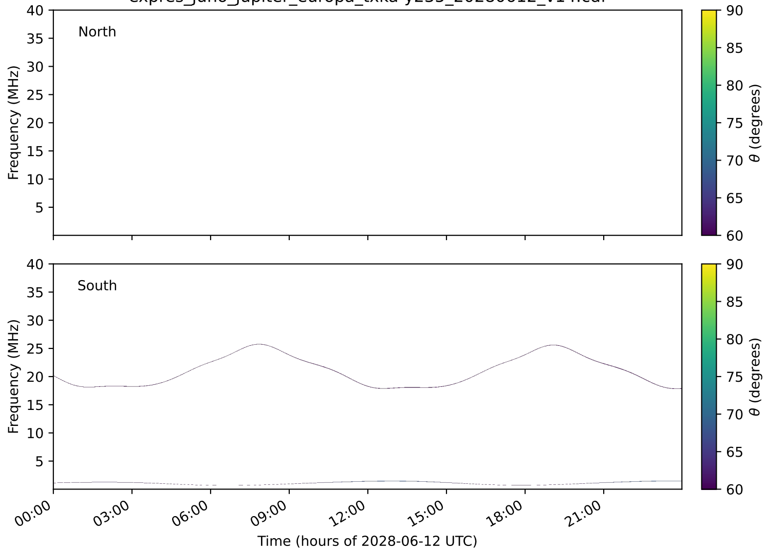
expres_juno_jupiter_europa_txka-y235_20280612_v14.cdf
