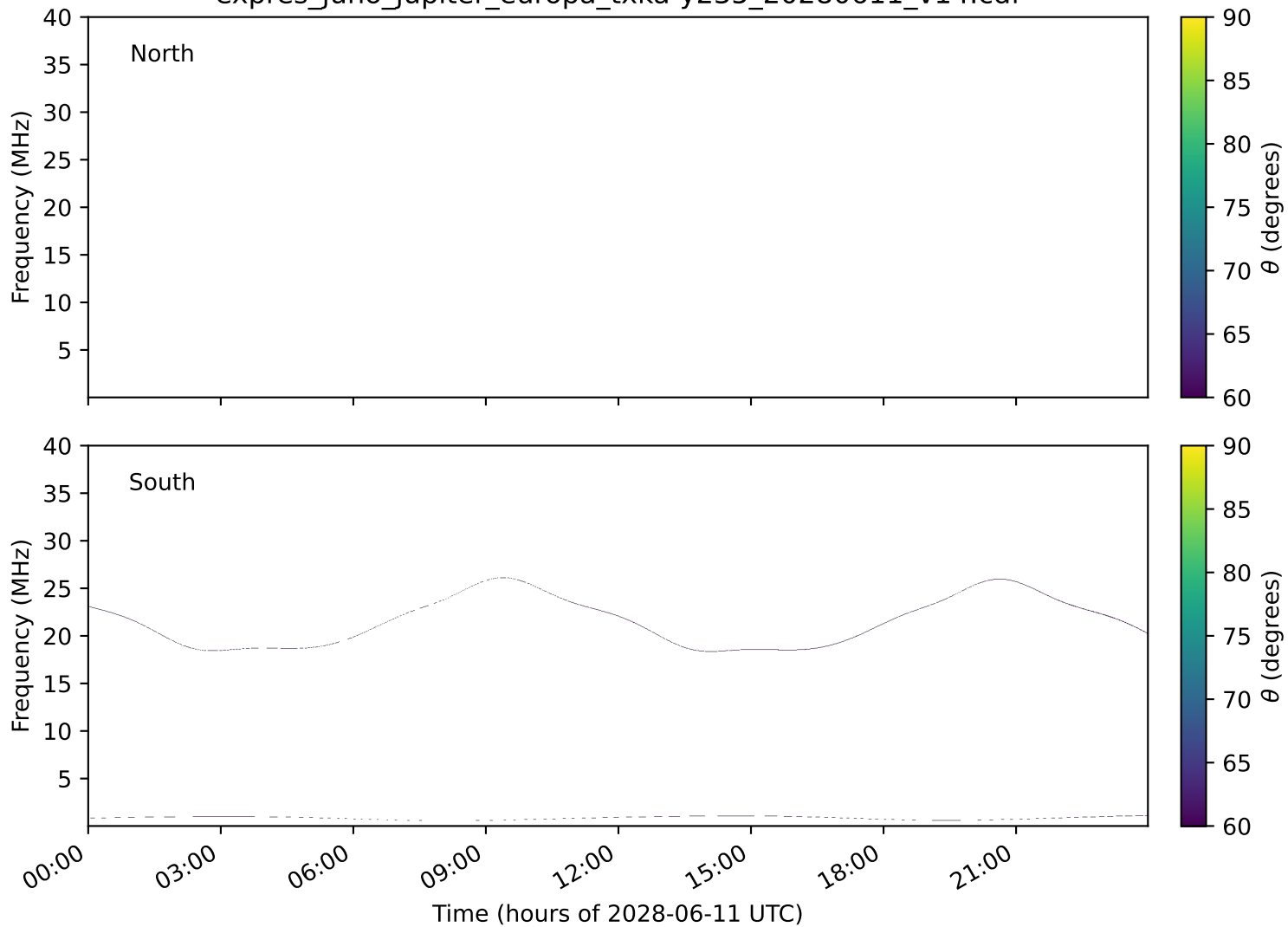
expres_juno_jupiter_europa_txka-y235_20280611_v14.cdf
