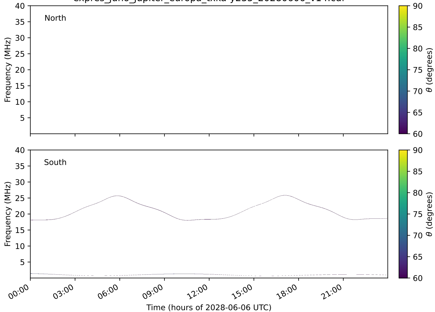
expres_juno_jupiter_europa_txka-y235_20280606_v14.cdf
