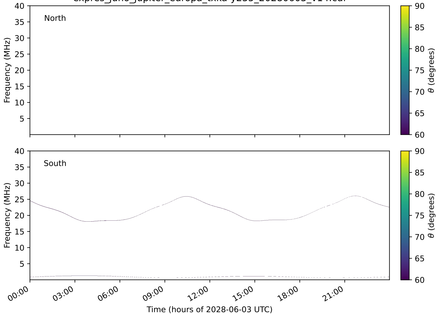
expres_juno_jupiter_europa_txka-y235_20280603_v14.cdf
