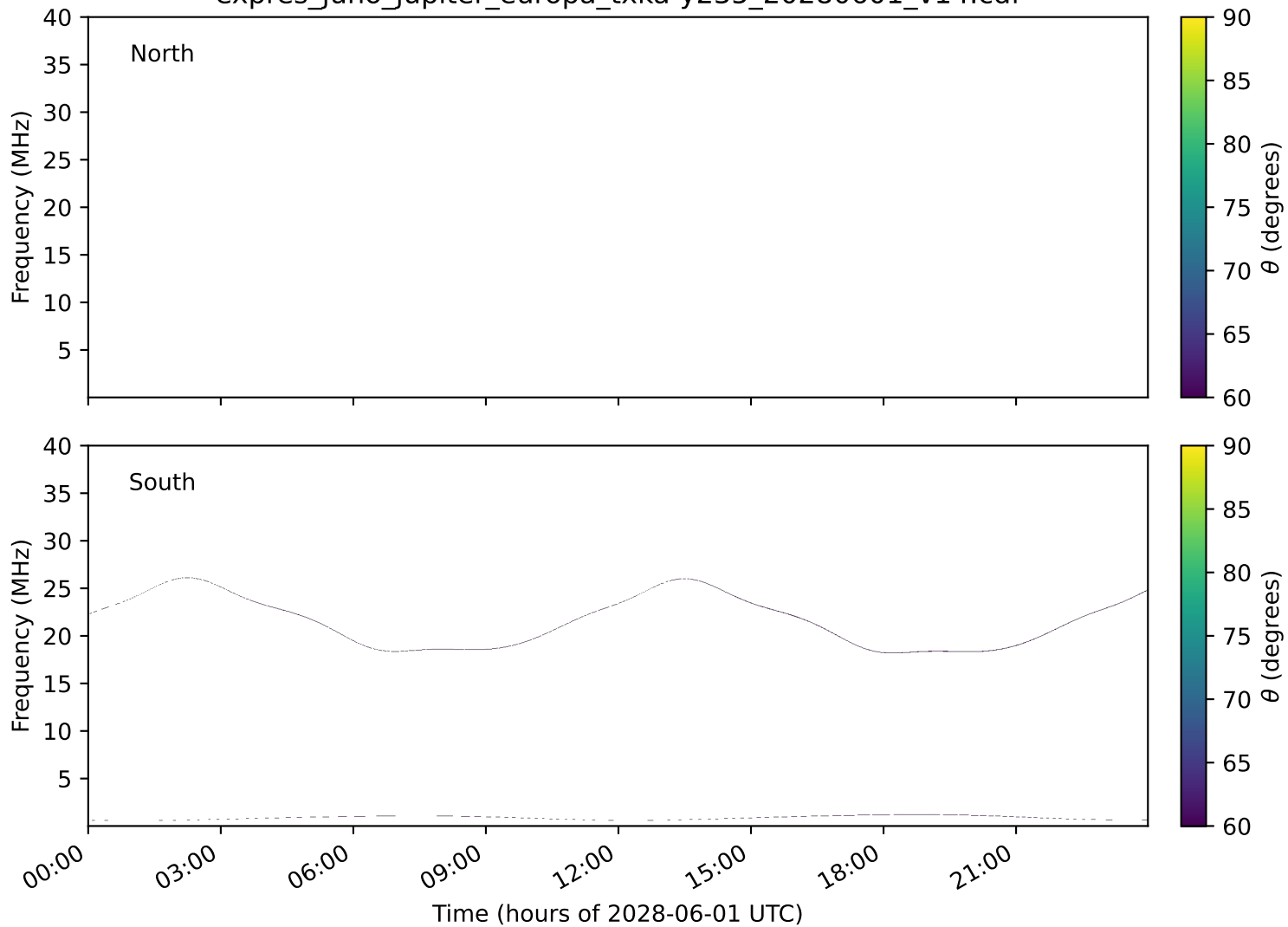
expres_juno_jupiter_europa_txka-y235_20280601_v14.cdf
