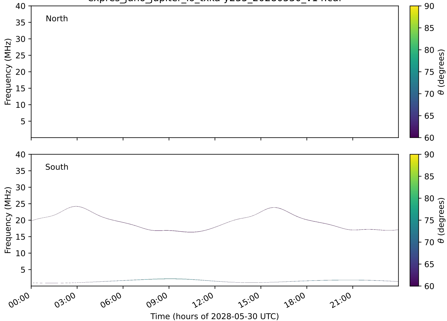
expres_juno_jupiter_io_txka-y235_20280530_v14.cdf
