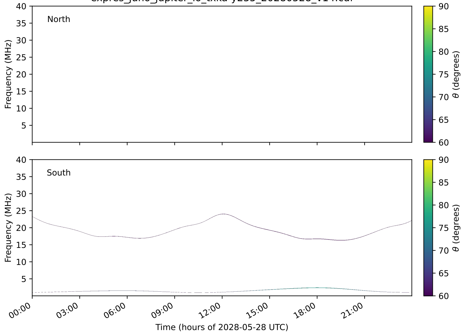
expres_juno_jupiter_io_txka-y235_20280528_v14.cdf
