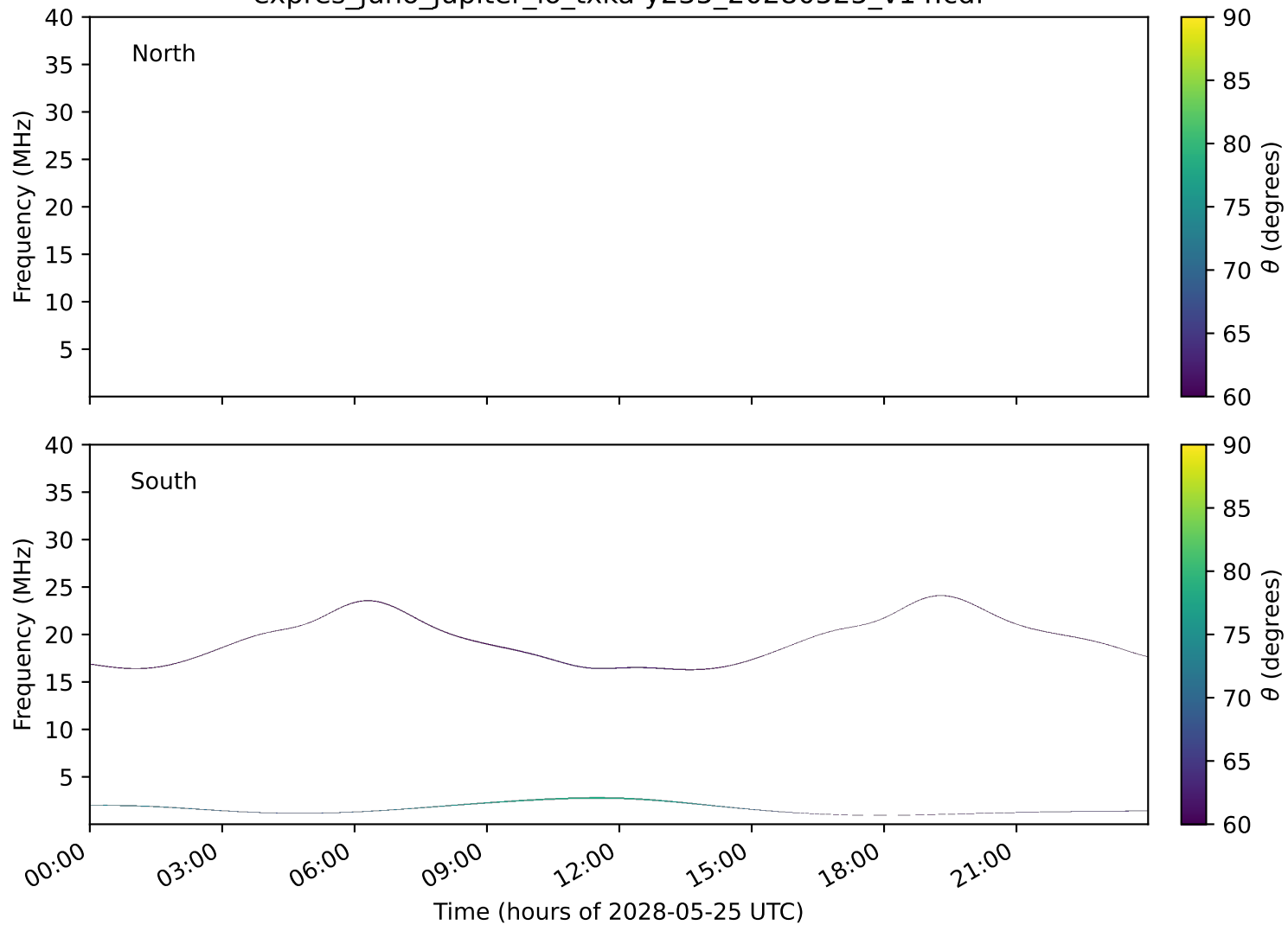
expres_juno_jupiter_io_txka-y235_20280525_v14.cdf
