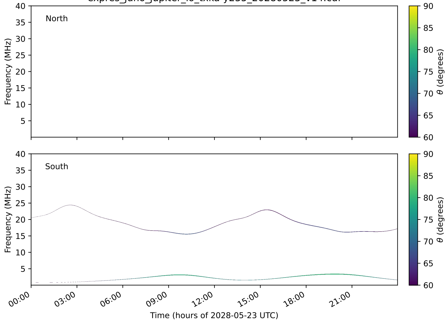
expres_juno_jupiter_io_txka-y235_20280523_v14.cdf
