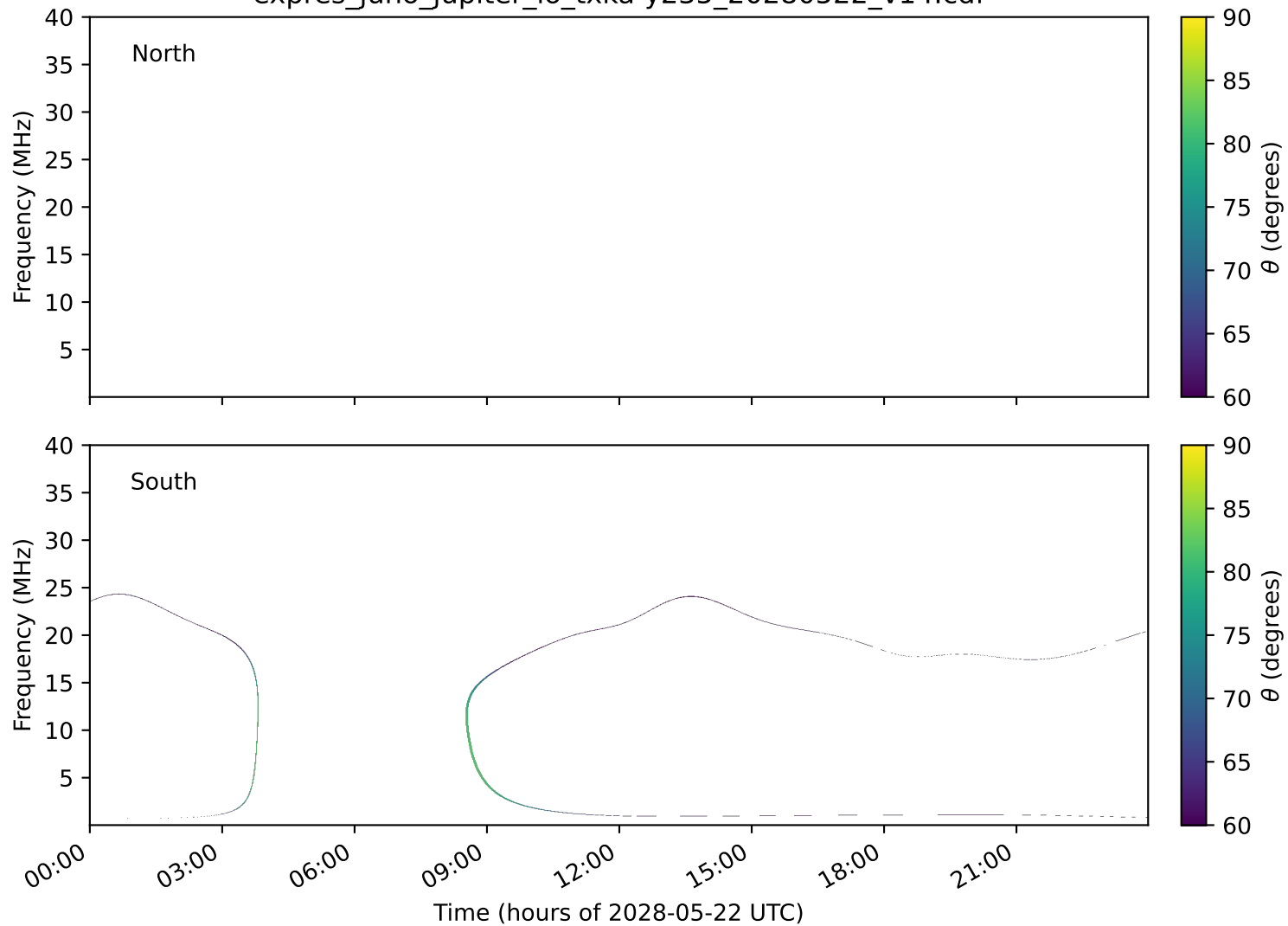
expres_juno_jupiter_io_txka-y235_20280522_v14.cdf
