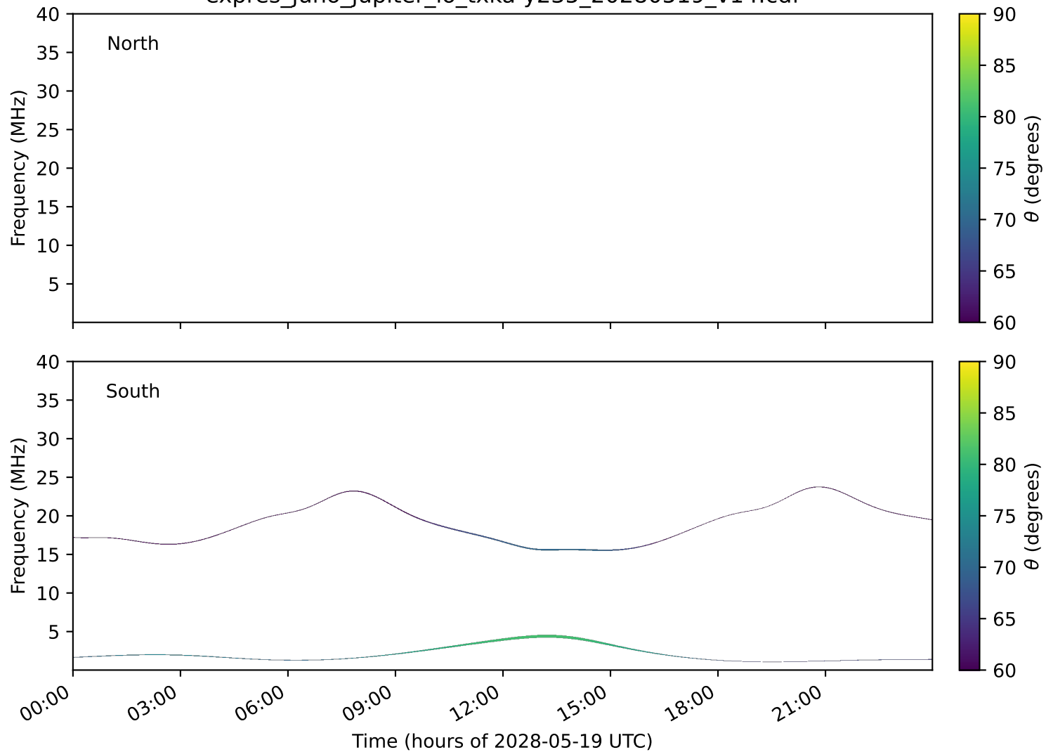
expres_juno_jupiter_io_txka-y235_20280519_v14.cdf
