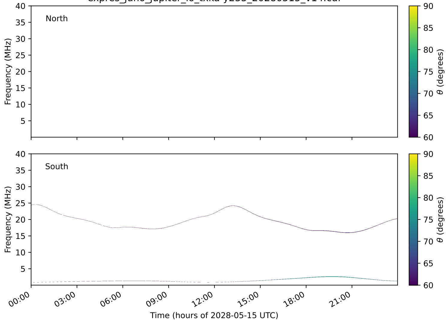
expres_juno_jupiter_io_txka-y235_20280515_v14.cdf
