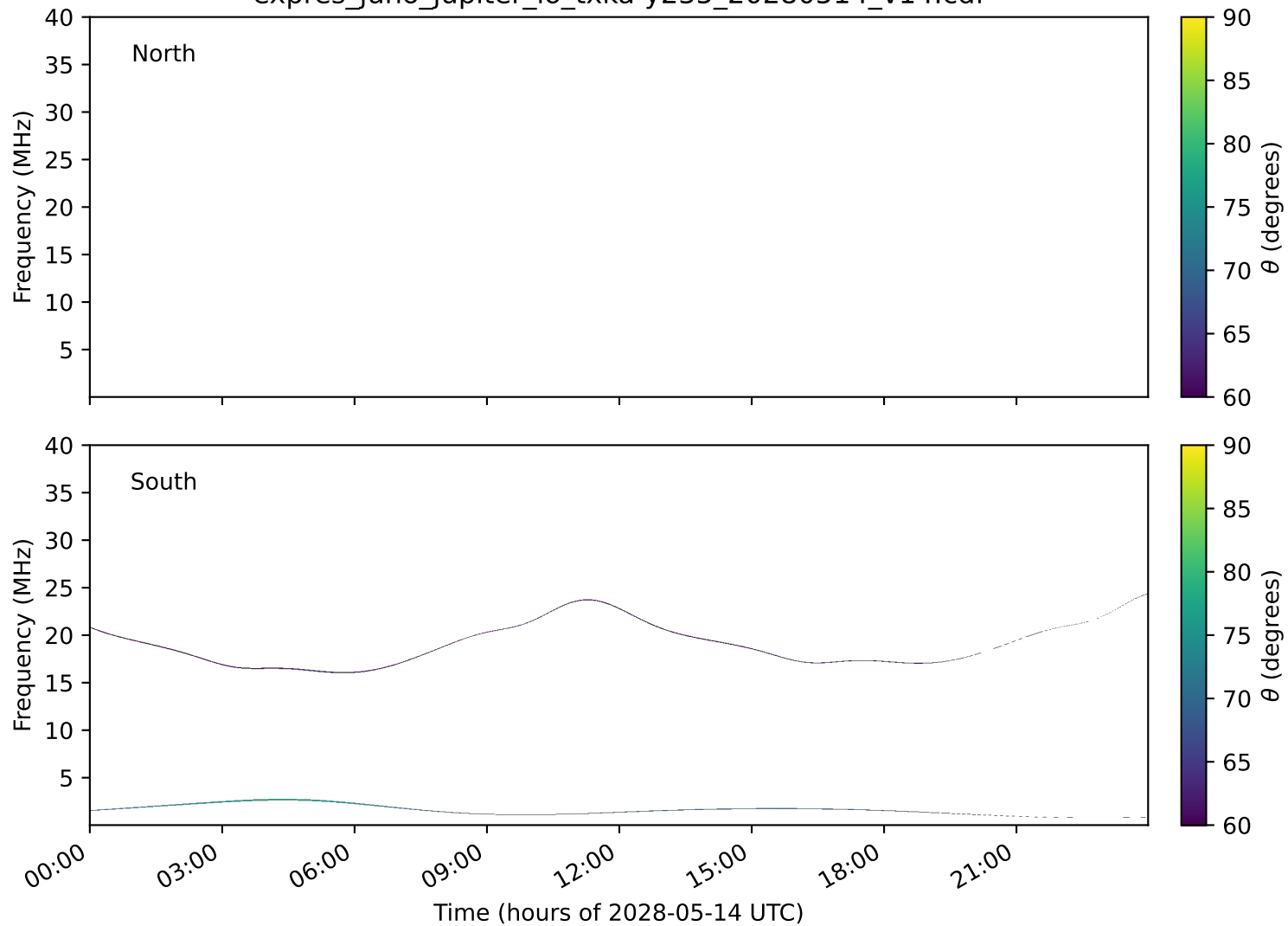
expres_juno_jupiter_io_txka-y235_20280514_v14.cdf
