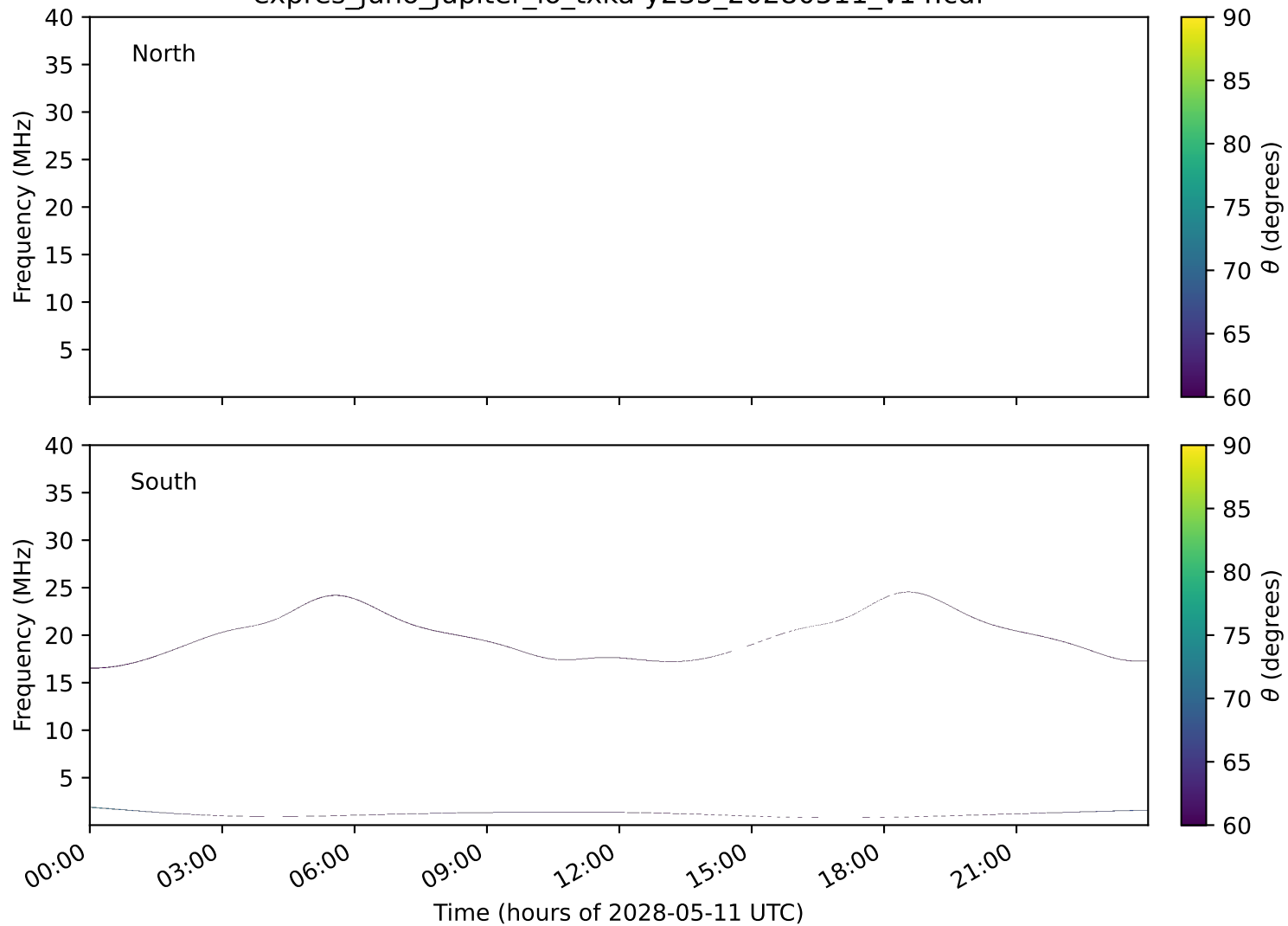
expres_juno_jupiter_io_txka-y235_20280511_v14.cdf
