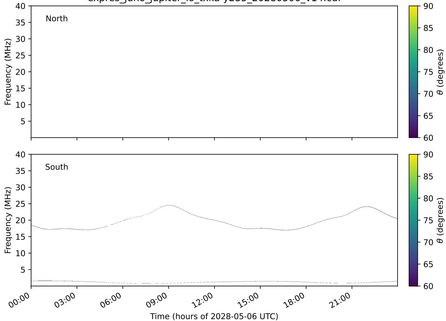
expres_juno_jupiter_io_txka-y235_20280506_v14.cdf
