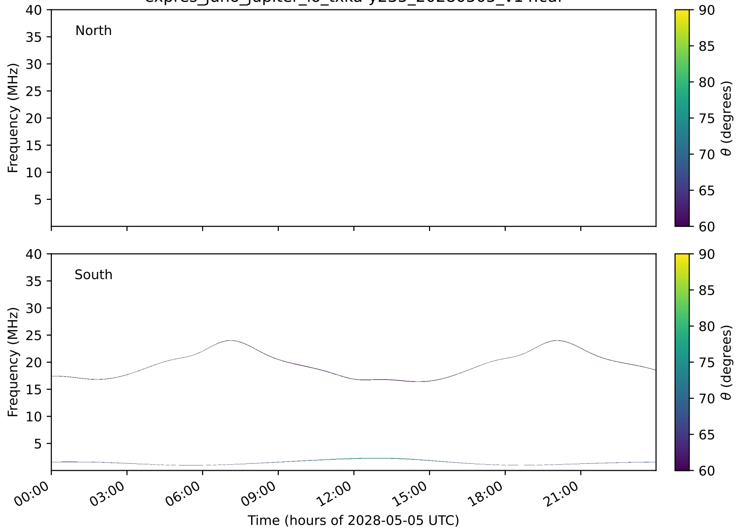
expres_juno_jupiter_io_txka-y235_20280505_v14.cdf
