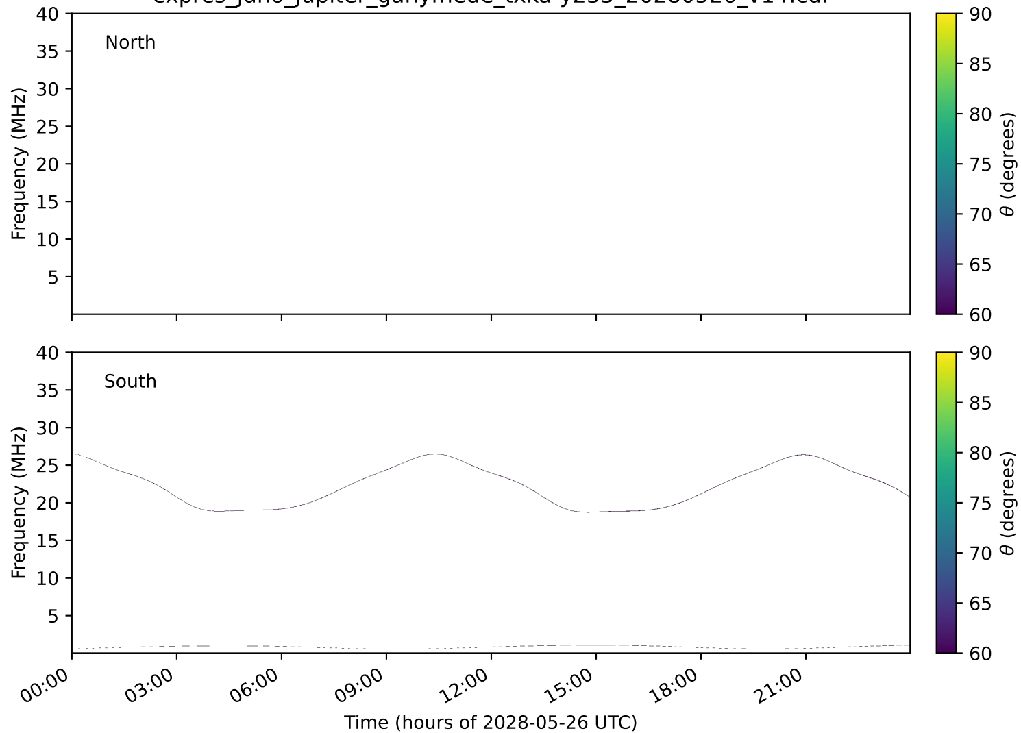
expres_juno_jupiter_ganymede_txka-y235_20280526_v14.cdf
