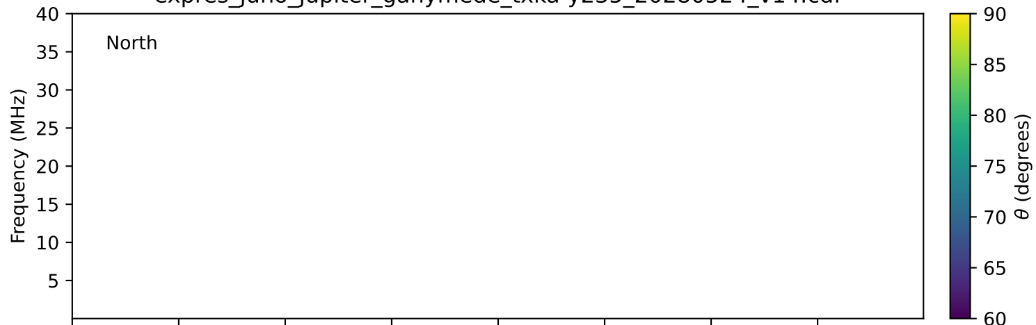
expres_juno_jupiter_ganymede_txka-y235_20280524_v14.cdf
