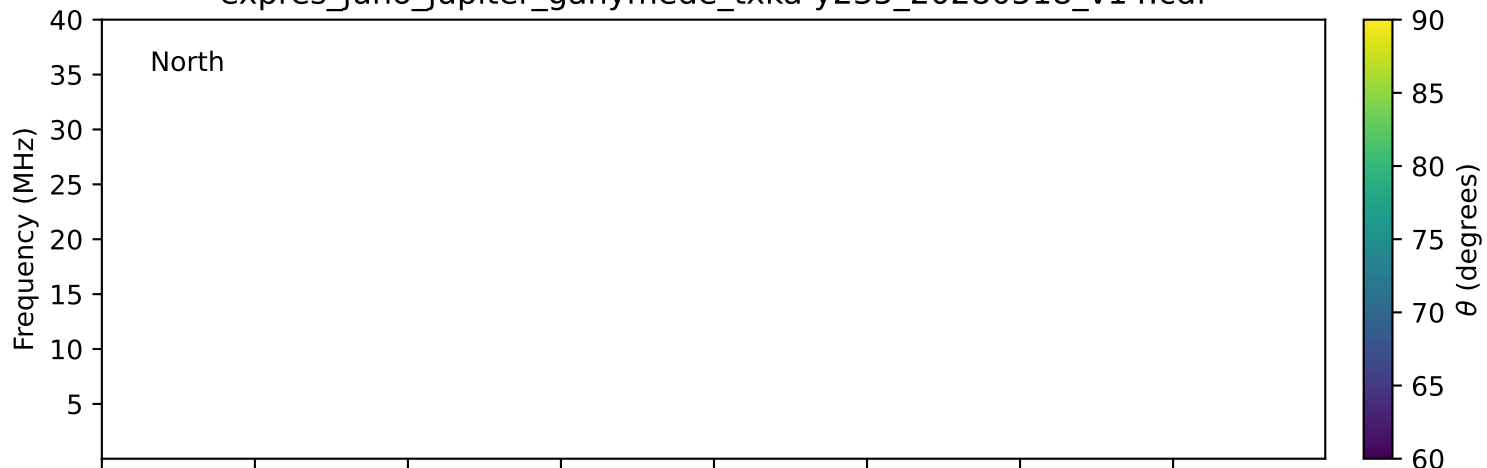
expres_juno_jupiter_ganymede_txka-y235_20280518_v14.cdf
