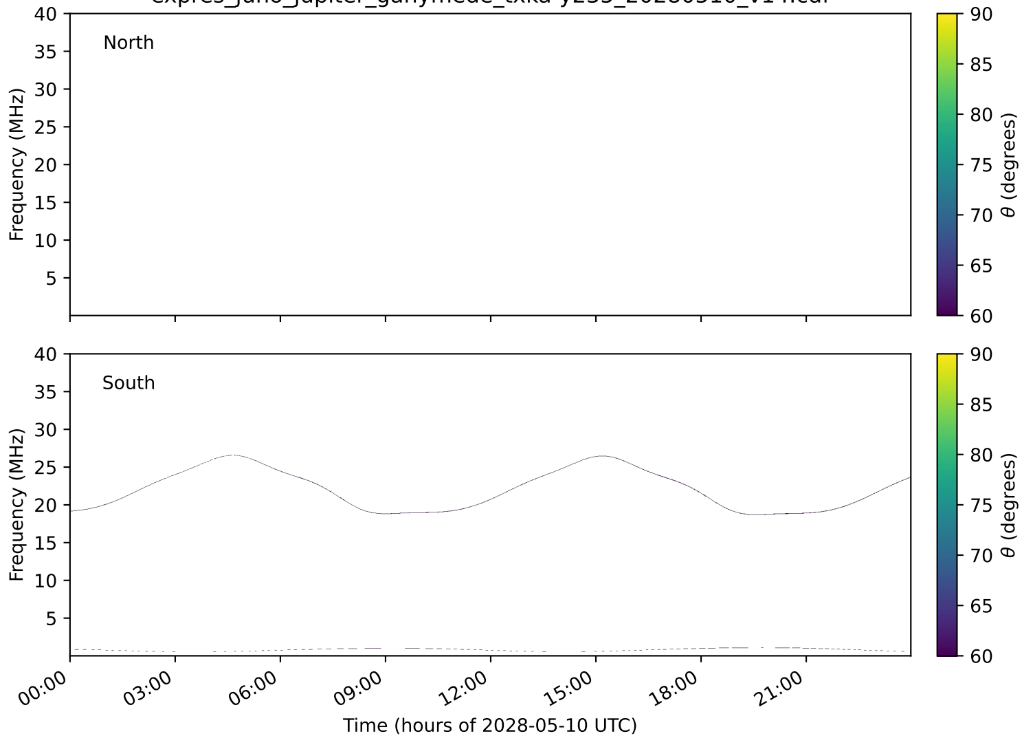
expres_juno_jupiter_ganymede_txka-y235_20280510_v14.cdf
