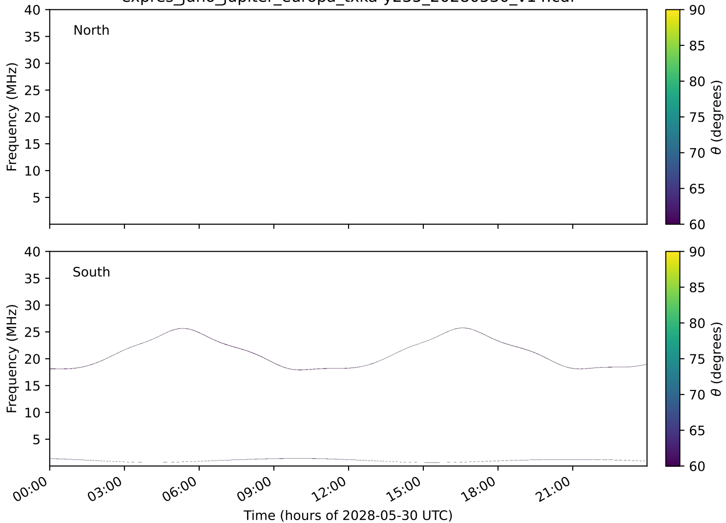
expres_juno_jupiter_europa_txka-y235_20280530_v14.cdf
