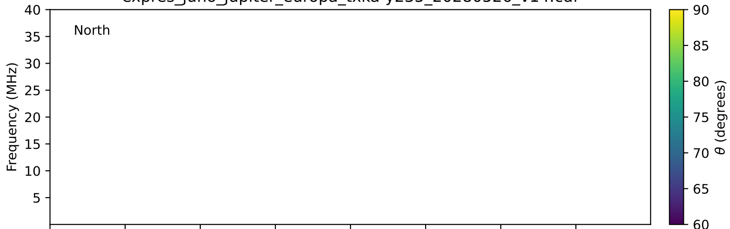
expres_juno_jupiter_europa_txka-y235_20280526_v14.cdf
