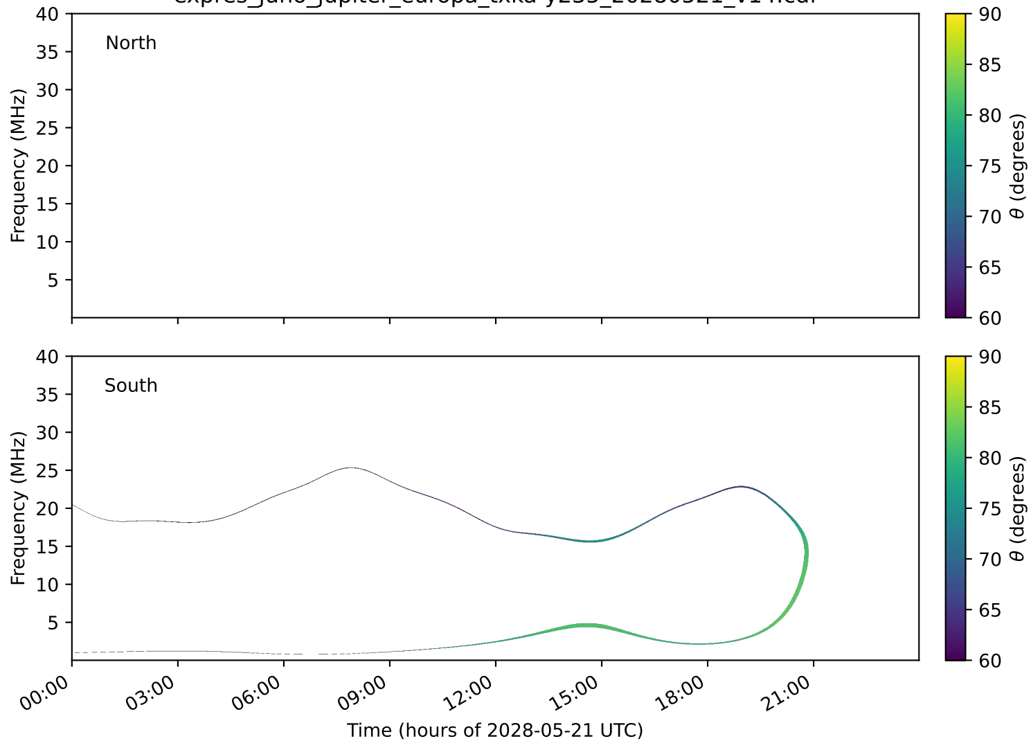
expres_juno_jupiter_europa_txka-y235_20280521_v14.cdf
