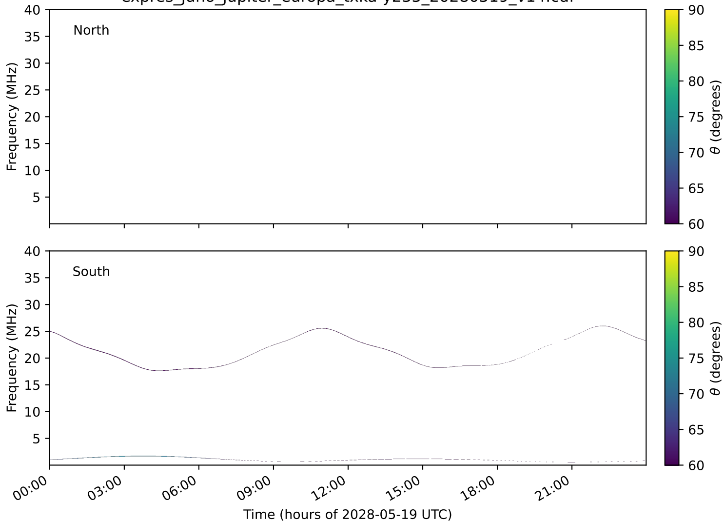
expres_juno_jupiter_europa_txka-y235_20280519_v14.cdf
