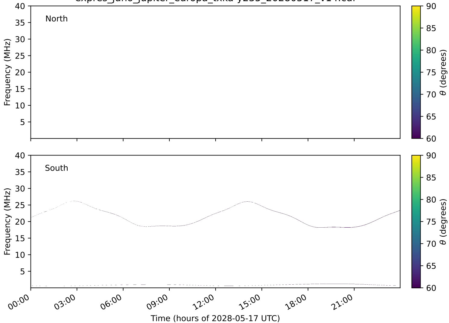
expres_juno_jupiter_europa_txka-y235_20280517_v14.cdf
